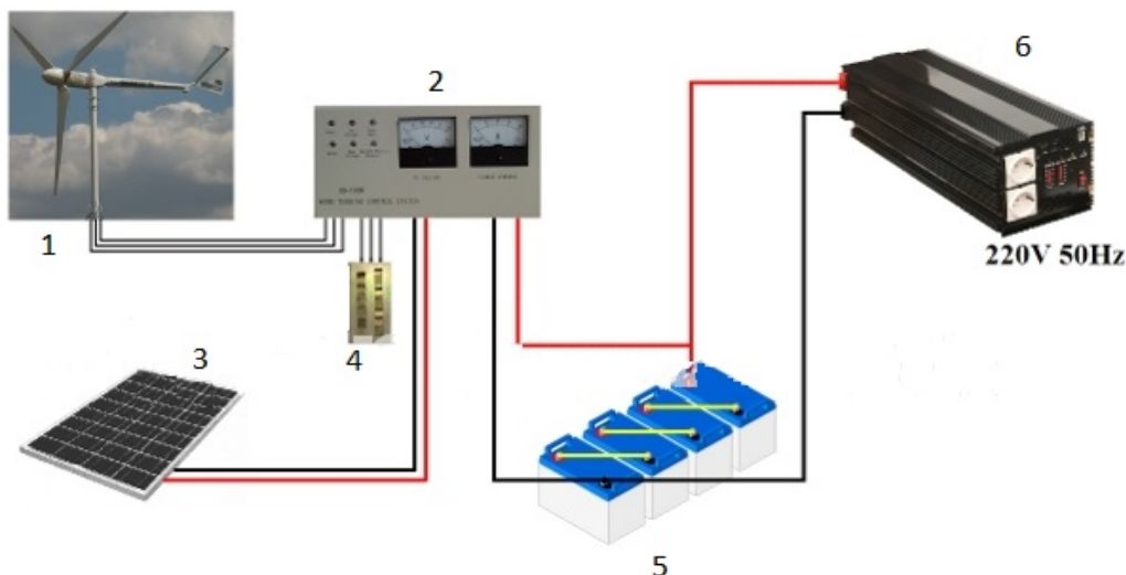
Figure 5. Components of hybrid system.
