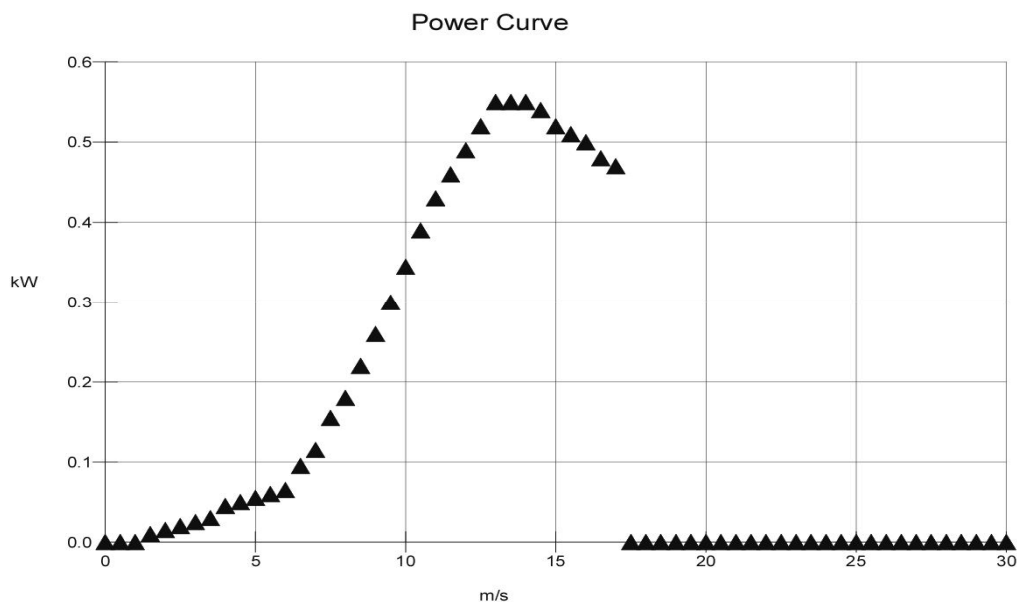
Figure 10. Power curve of the wind generator from hybrid system
