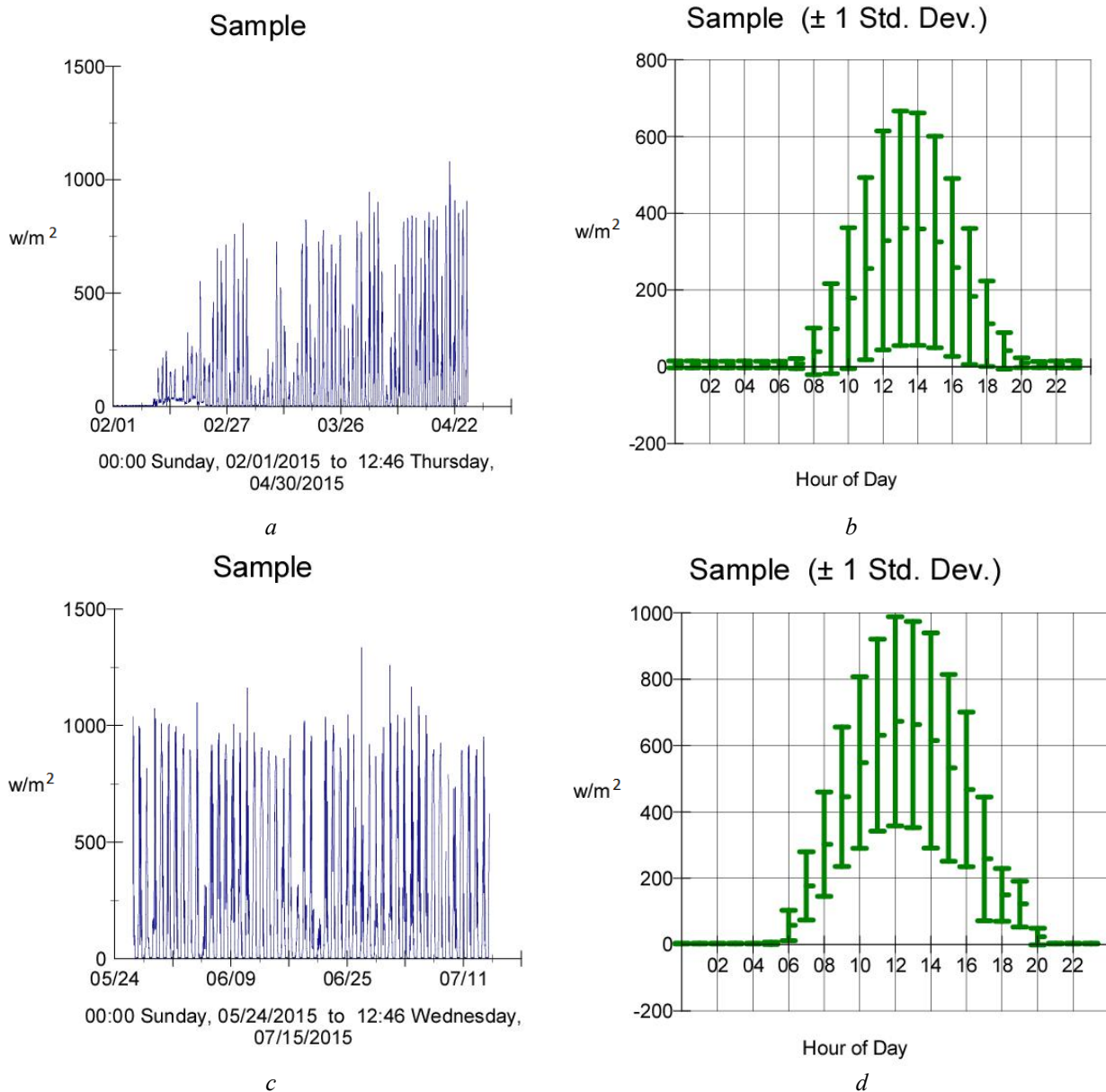
Figure 11. Solar radiation data for winter - a, b and summer season - c, d
