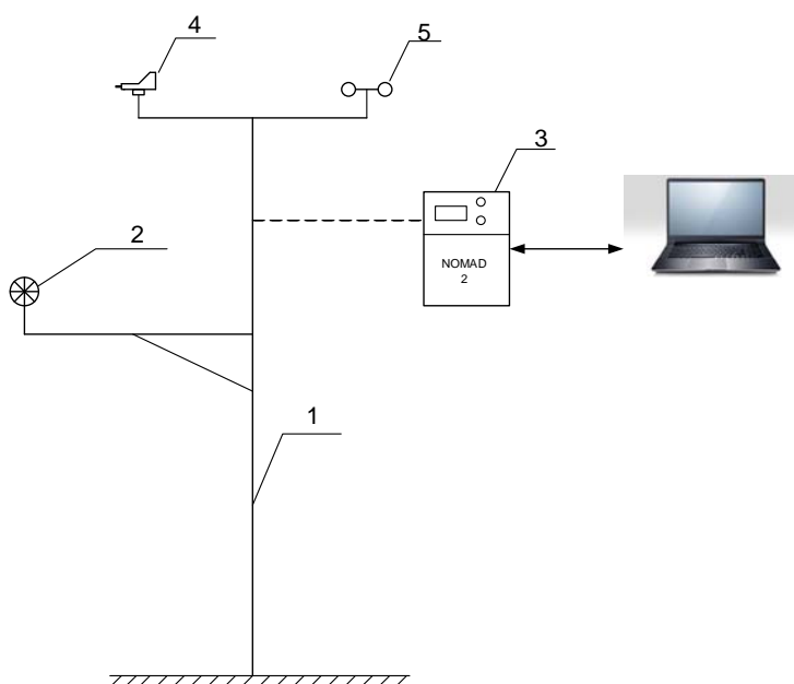
Figure 1. Scheme of equipment for measuring wind parameters
